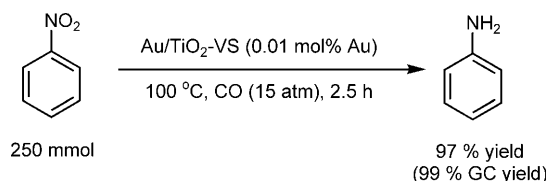
Scheme 1. Reduction of nitrobenzene on a 250 mmol scale.
